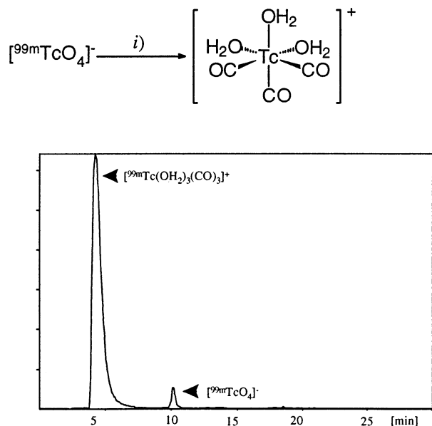
Fig. 2. Reaction conditions for the preparation of 1a' : (i) generator eluate up to 37 GBq [^{99m}\text{TcO}_4]^- , 0.9% NaCl/ \text{H}_2\text{O} , \text{NaBH}_4 , vial filled with CO, 25 min 75^\circ\text{C} (above); HPLC trace of the crude reaction mixture (below).
