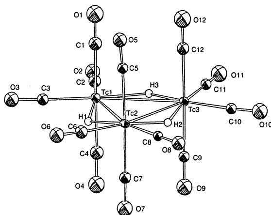
Fig. 1. ORTEP presentation of the mixed hydrido-carbonyl complex [\text{H}^{99\text{m}}\text{Tc}(\mu\text{-H})_3(\text{CO})_4]_3^- .
