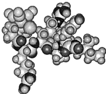
Fig. 9. Calculated structure of [\text{TcCl}(\text{CO})_3(\text{His}-\text{Arg}-\text{Arg}-\text{Pro}-\text{Tyr}-\text{Ile})] for relative size comparison and orientation. The fac - \text{Tc}(\text{CO})_3 moiety is in the upper left corner of the peptide.
