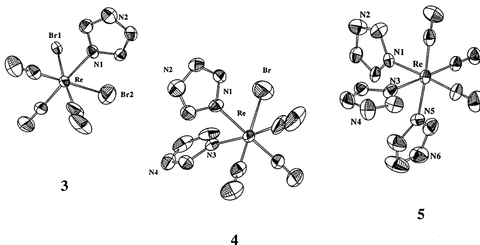
Fig. 3. ORTEP presentations of the three different imidazole complexes [\text{Re}(\text{Br})_2(\text{im})(\text{CO})_3]^- ( 3 ), [\text{ReBr}(\text{im})_2(\text{CO})_3] ( 4 ) and [\text{Re}(\text{im})_3(\text{CO})_3]^+ ( 5 ).
