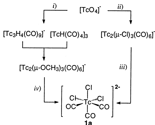
Scheme 2. Low pressure carbonylation of [^{99}TcO_4]^- , in general: r.t., 1 atm CO, THF·BH 3 : (i) no Cl - ; (ii) with Cl - ; (iii) excess Cl - ; and (iv) NaOH in CH 3 OH then HCl.
